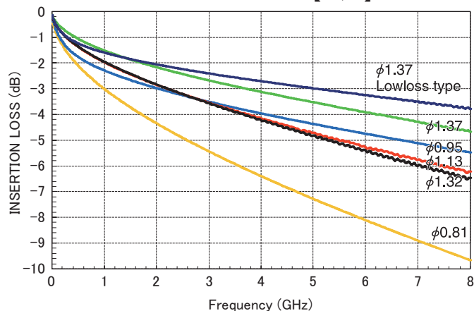
Insertion Loss comparison between each cable size【dB/m】
