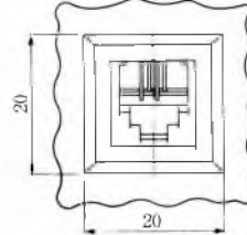
Panel mounting dimensions
