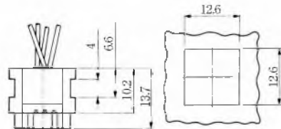
Panel mounting dimensions
